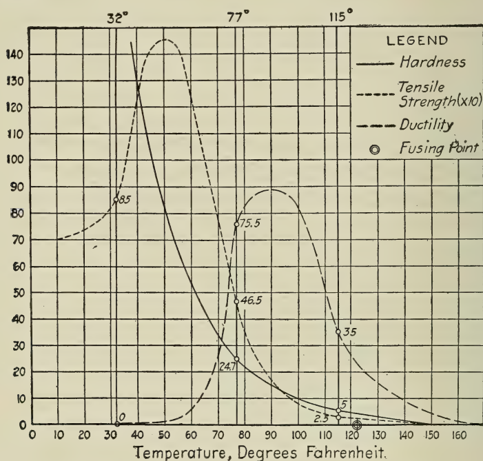
FIG. 100.—Chart of Physical Characteristics of Coal-tar Pitch.
